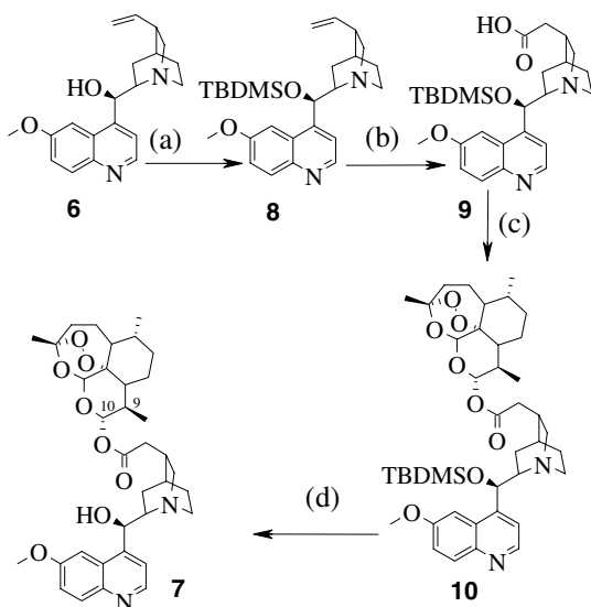
Scheme 1. Reagents and conditions: (a) TBDMSO, Et 3 N, DMAP, DMF, rt; (b) i-BH 3 -THF, diglyme, 0 °C; ii—Me 3 NO-2H 2 O, 100 °C; iii—Jones reagent, acetone, rt; (c) i—2,6-dichlorobenzoyl chloride, Et 3 N, DMAP, DCM, rt; (d) TBAF, THF, rt.
